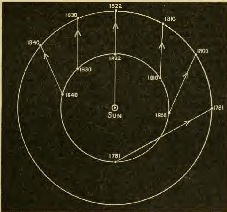
THE MOVEMENT OF URANUS AND NEPTUNE.
